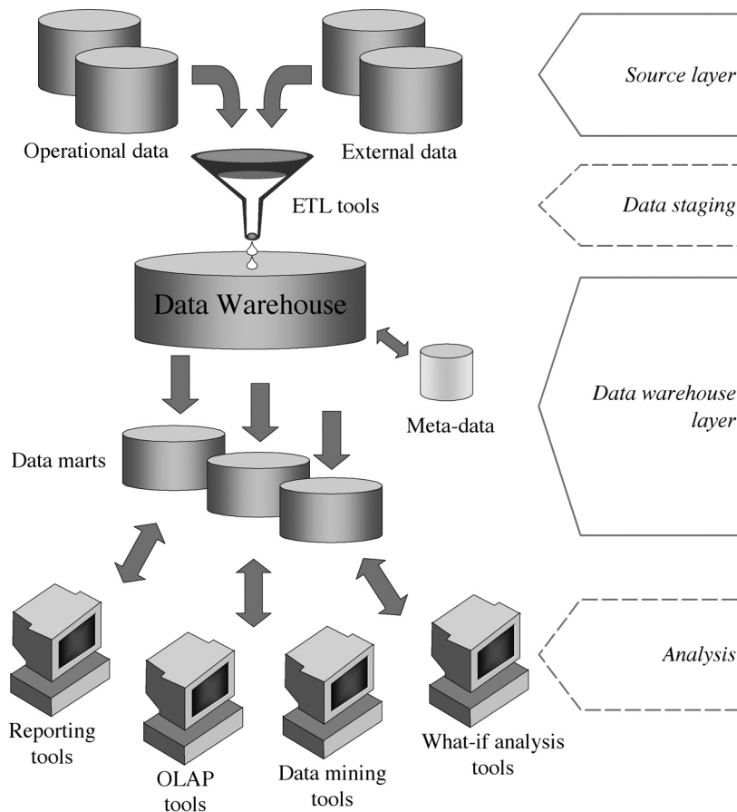
FIGURE 1-3 Two-layer architecture for a data warehouse system
