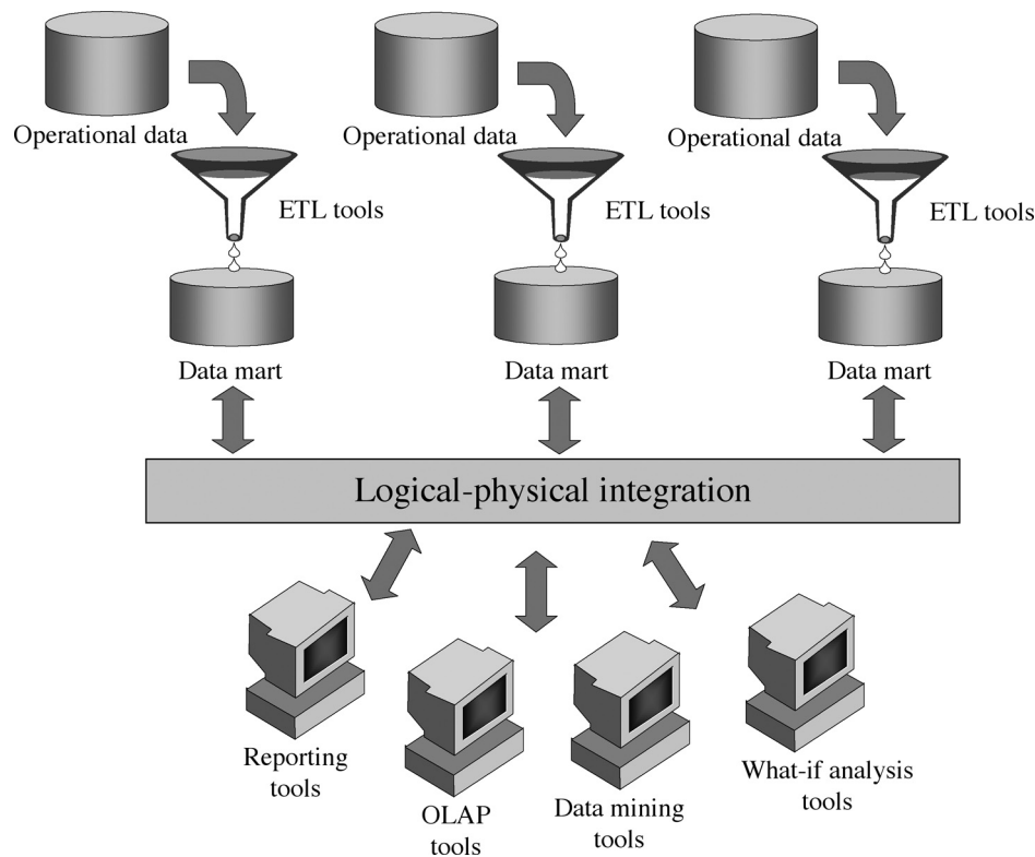
FIGURE 1-7 Federated architecture
