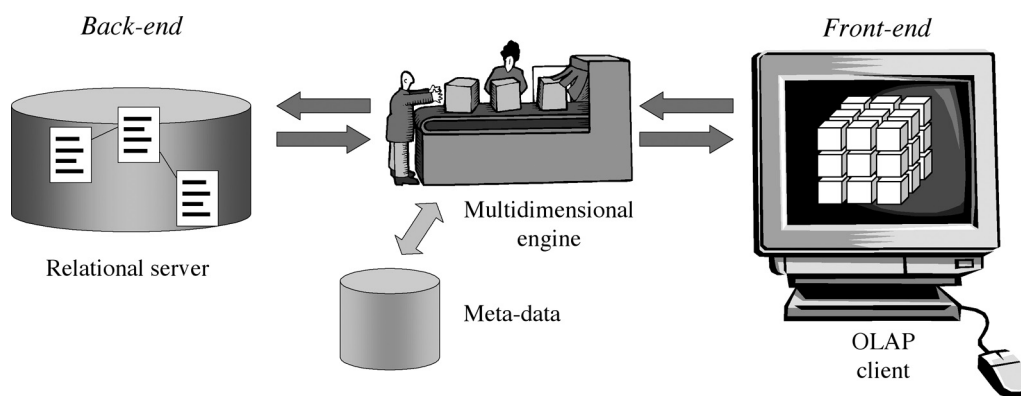
FIGURE 1-32 ROLAP architecture
