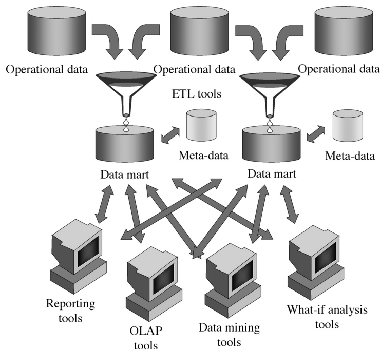
FIGURE 1-5 Independent data marts architecture
