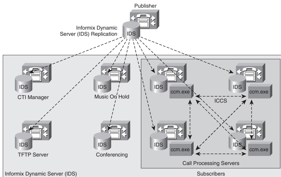
Figure 1-5 CUCM Cluster
