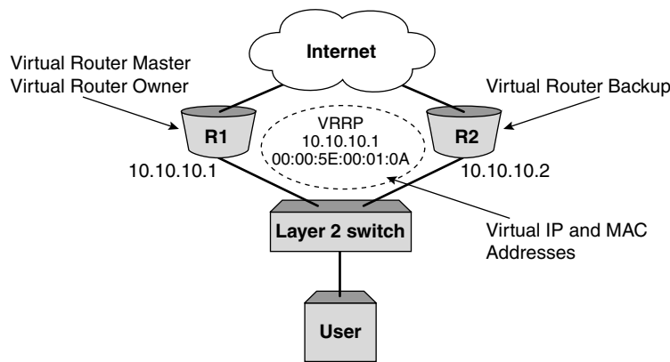
Figure 2-14 VRRP addressing example topology.
